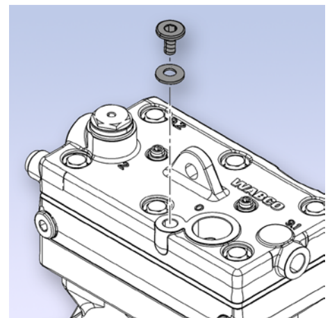
Closing port 4 of the compressor
